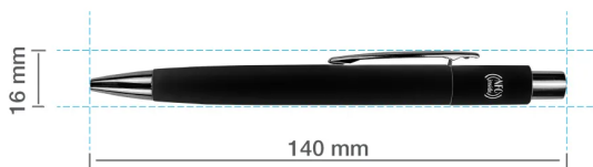
NFC-PN-01 Dimensions
